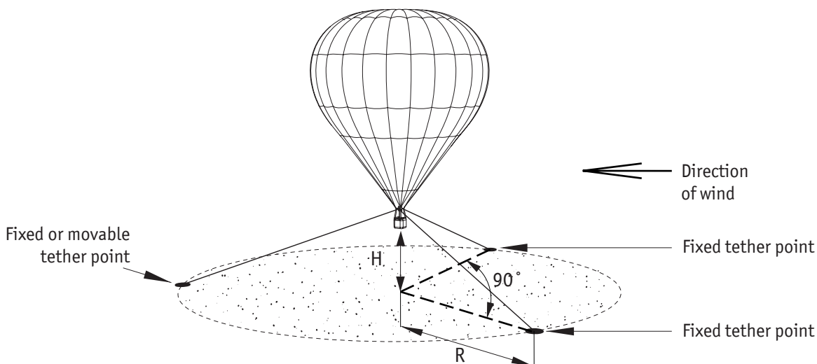
Tether layout
